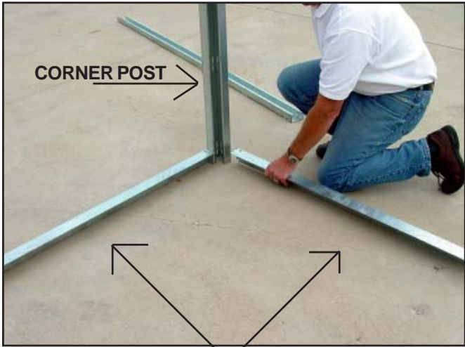
CROSS BARS
